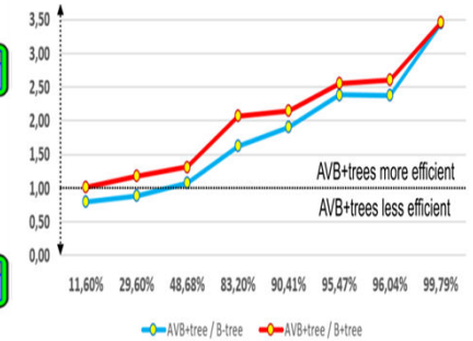
AVB+tree/B-tree AVB+tree/B+tree
