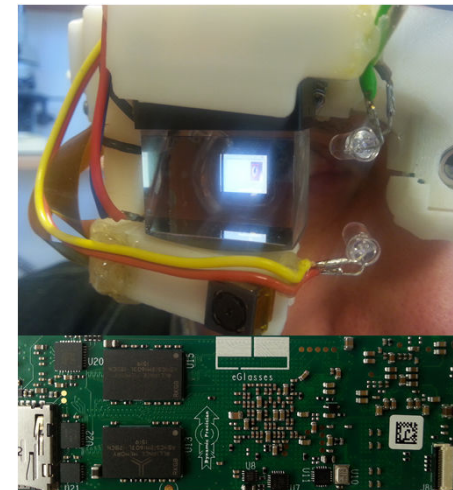
The eGlasses prototype
